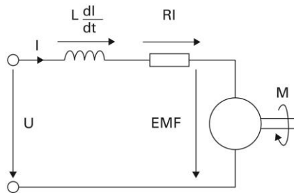
Fig. 3 Simplified rotor circuit equivalent diagram of a DC motor with inductance, resistor of the rotor winding, and rotor voltage.
