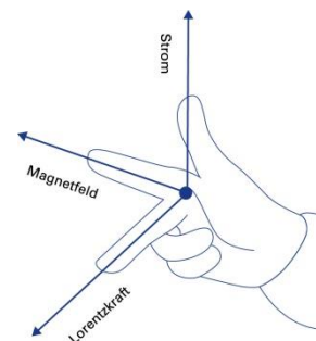
Fig. 1 With the help of the right-hand-rule, it is possible to establish the direction of the force relative to the direction of the current and the magnetic field.
